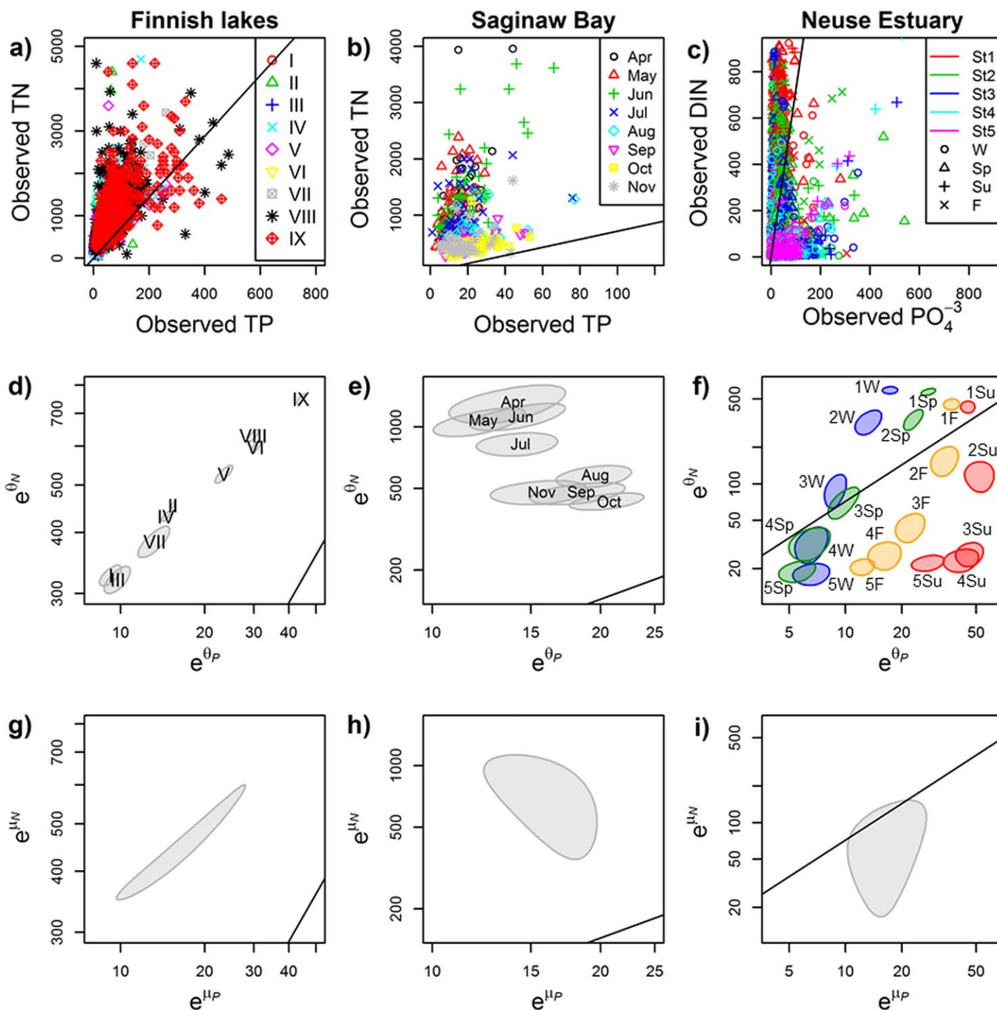
Fig. 2. Relationships between N ( \mu\text{g/L} ) and P ( \mu\text{g/L} ) concentrations for (a, d, g) Finnish lakes, (b, e, h) Saginaw Bay, and (c, f, i) the Neuse Estuary. In panels (a-c) color-symbol combinations, marked differently by group, denote individual observations. In panels (d-f) ellipses denote the 95% contour of joint distribution of group N and P from the BIBM. In panels (g-i) ellipses denote the 95% contour of joint distribution of overall system N and P from the BIBM. In all panels, solid diagonal lines indicate the Redfield ratio (mass N:P = 7.2:1). In panels (f), abbreviations are the combination of section and season: the number indicates the sections 1-5 and the text indicates the season (W: Winter, Sp: Spring, Su: Summer, and F: Fall).
