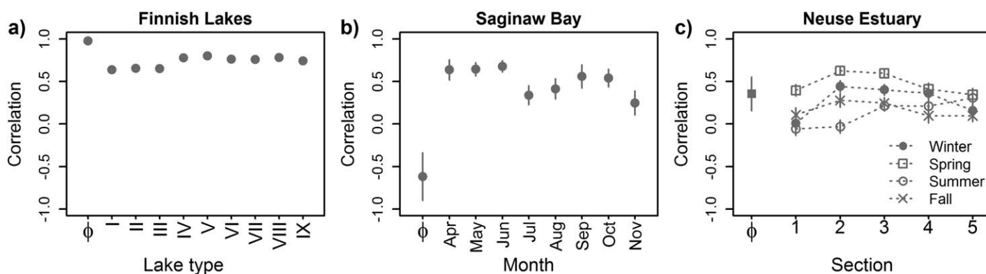
Fig. 3. Cross-group ( \phi ) and within-group ( \rho ) correlation between N and P for (a) Finnish lakes and (b) Saginaw Bay, and (c) the Neuse Estuary. Gray symbol and gray vertical line denote the mean and 95% interval estimated using the Bayesian hierarchical model.
