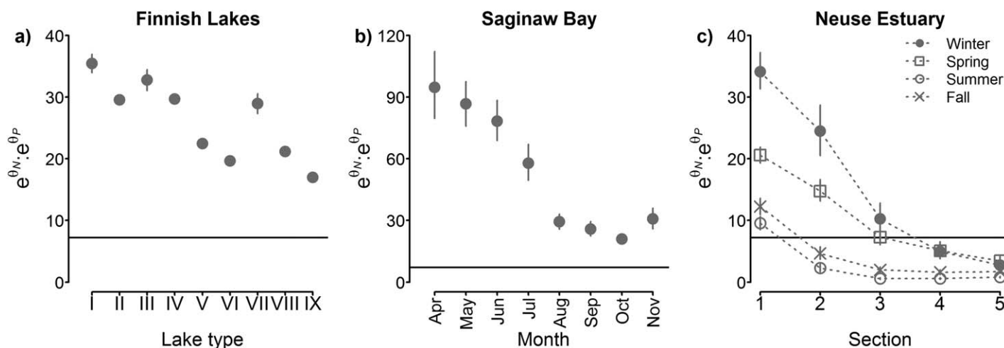
Fig. 4. Group N:P distribution for (a) Finnish lakes, (b) Saginaw Bay, and (c) Neuse Estuary. Gray circle and gray vertical line denote the median and 95% interval estimated using the Bayesian hierarchical model. Solid horizontal line indicates the Redfield ratio (mass N:P = 7.2:1).
