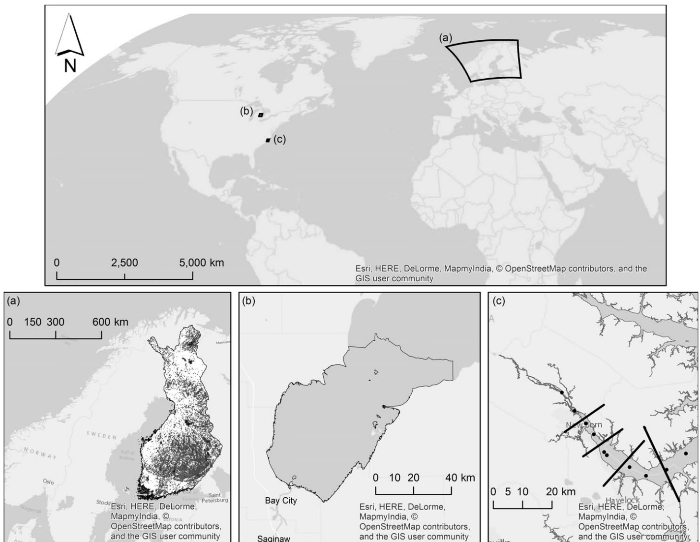
Fig. 1. (a) Finnish lakes, (b) Saginaw Bay, Lake Huron Michigan, (c) Neuse Estuary, North Carolina; also showing the monitoring stations (black circle) with respect to the five estuarine sections of the Neuse, which are delineated with black lines.
